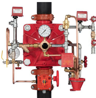
Deluge Valve
